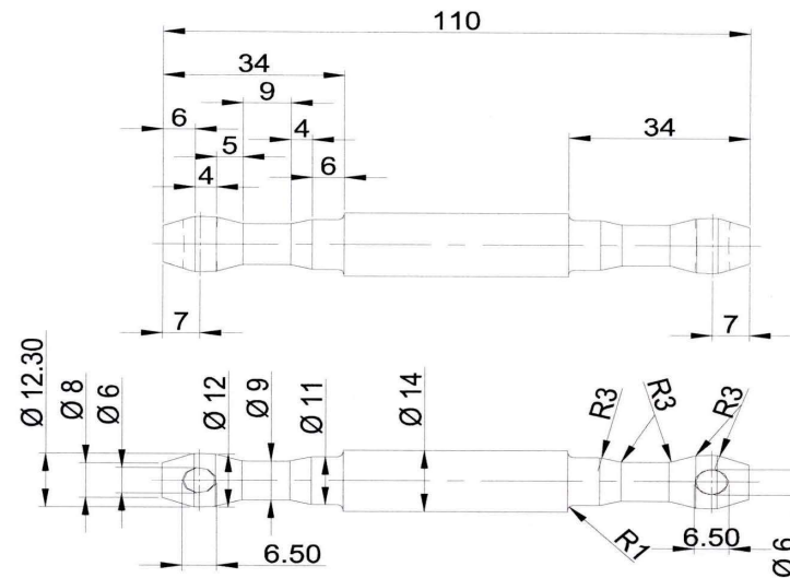
2 COUPLING SHAFT FOR NM 15
